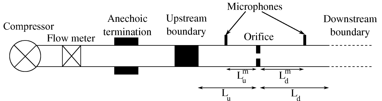
FIG. 6.3: Scheme of the test rig
