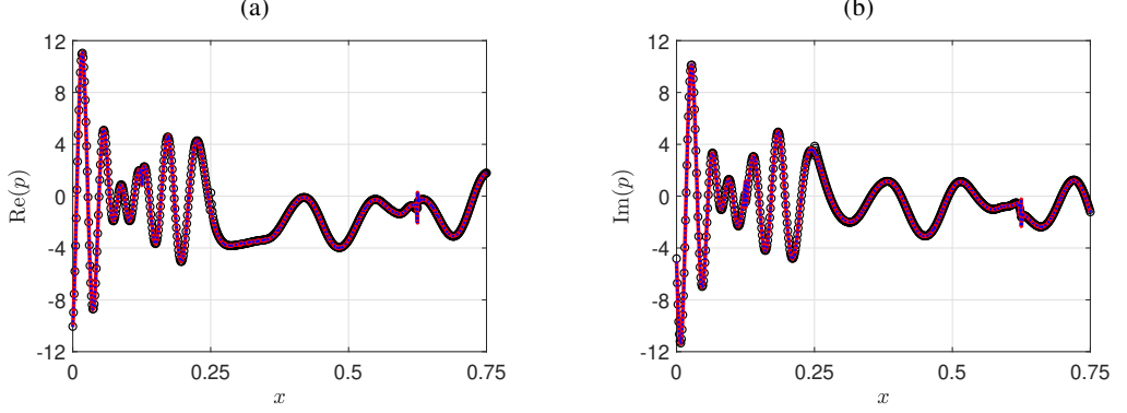
Figure 6: (a) Real part and (b) imaginary part of the pressure field at f = 5 kHz along the lined duct top wall ( y = h_d ): \cdots Pierce's equation, \text{—} Goldstein's equation and \circ mode-matching results (reference).
