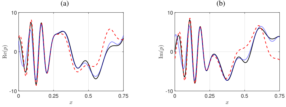
Figure 10: (a) Real part and (b) imaginary part of the pressure field at f = 5 kHz along the duct top wall ( y = h_d ): — LEE, · · · · Pierce's equation and - - - Goldstein's equation.
