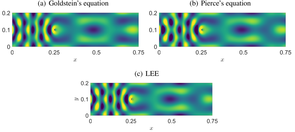
Figure 9: Real part of pressure in the duct with sheared flow at f = 5 kHz. (a) Goldstein's equation, (b) Pierce's equation and (c) LEE. Levels between -7 Pa and +7 Pa from blue to yellow.
