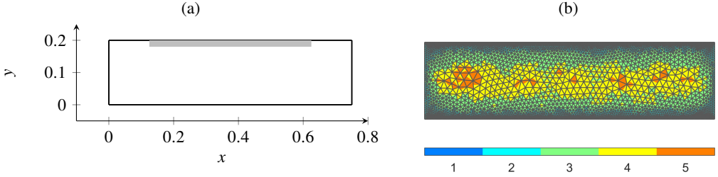
Figure 4: (a) Computational domain with liner in gray and (b) mesh with FEM face order distribution at f = 5 kHz.
