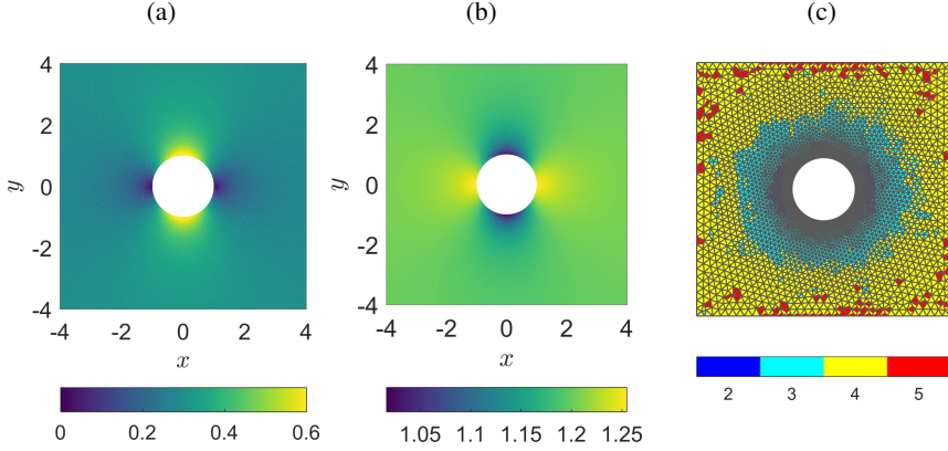
Figure 1: Computational domain: (a) mean Mach number, (b) mean density and (c) mesh with FEM face order distribution for \omega = 10c_0/R .
