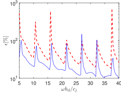
Figure 11: Relative error with respect to the LEE solution for the acoustic pressure along the duct top wall ( y = h_d ): · · · · Pierce's equation and - - - Goldstein's equation.
