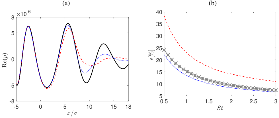
Figure 8: (a) Real part of the acoustic pressure at y = 6\sigma for St = 0.5 and (b) corresponding relative error \epsilon (with LEE as reference) for an increasing Strouhal number: — LEE, ···· Pierce's equation and - - - Goldstein's equation. Error levels for an isothermal jet with T_0 = 600 K are also reported for \times Pierce's equation and \circ Goldstein's equation.
