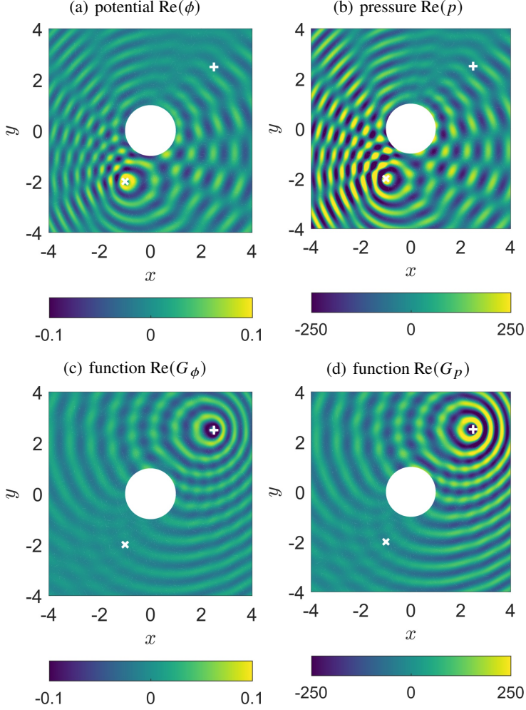
Figure 2: Real parts of the acoustic potential (a) and pressure (b) obtained with the direct problem for Goldstein's equation. Real parts of the numerical Green's functions (c) G_\phi and (d) G_p obtained from the corresponding adjoint problem, at \omega = 10c_\infty/R . \times : source location and + : observer position.
