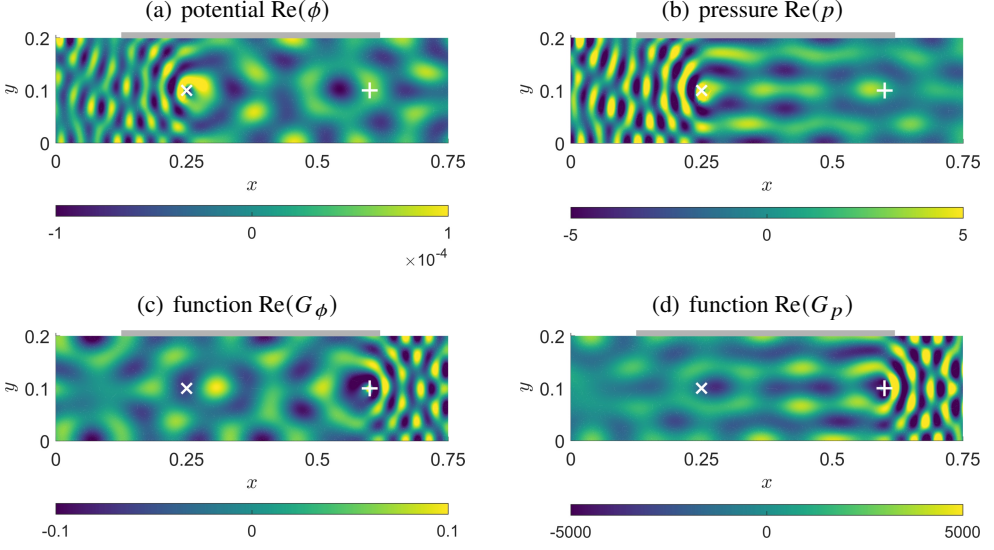
Figure 5: Real parts of the acoustic potential (a) and pressure field (b) obtained for Goldstein's equation, and real parts of the corresponding numerical Green's functions G_\phi (c) and G_p (d) obtained from the adjoint problem at f = 5 kHz. \times : source location and + : observer location. The liner is indicated in gray.
