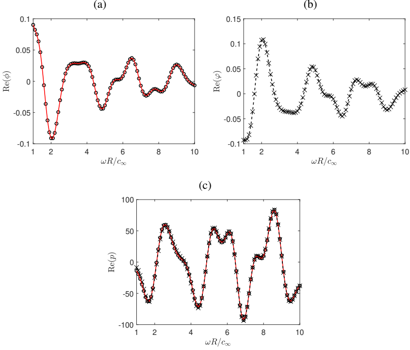
Figure 3: Real part of (a) the acoustic potential \phi , (b) the acoustic potential \varphi and (c) the acoustic pressure computed at x = y = 2.5R from: \circ Goldstein's direct problem, \times Pierce's direct problem, — Goldstein's adjoint problem and - - Pierce's adjoint problem.
