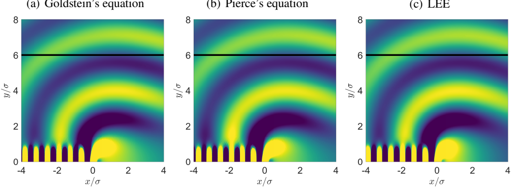
Figure 7: Real part of the pressure field for the hot jet problem at St = 0.5 obtained with (a) Goldstein's equation, (b) Pierce's equation and (c) the LEE. Levels between -10^{-5} Pa and 10^{-5} Pa from blue to yellow.
